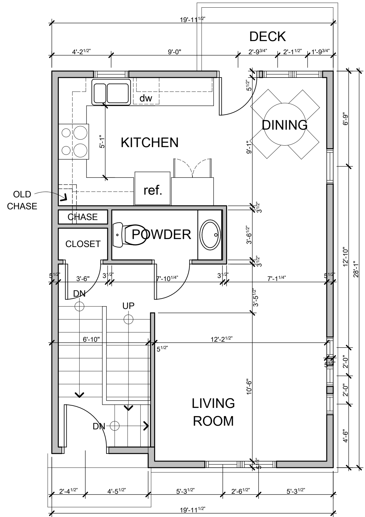
E4 Main Plan
