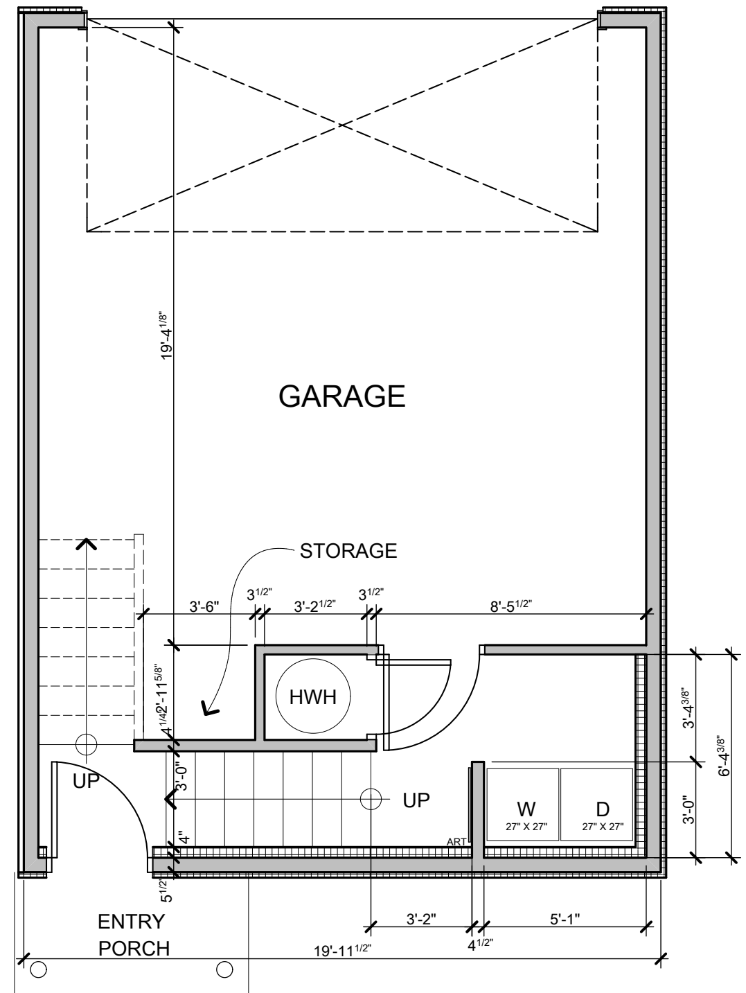
E4 Lower Plan
